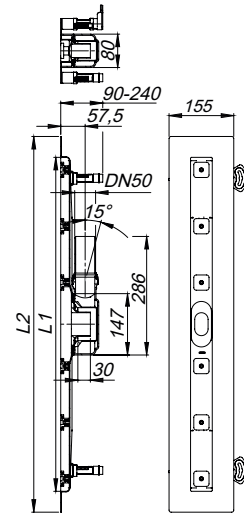
shower channel CeraLine Plan F 500 – 1200
