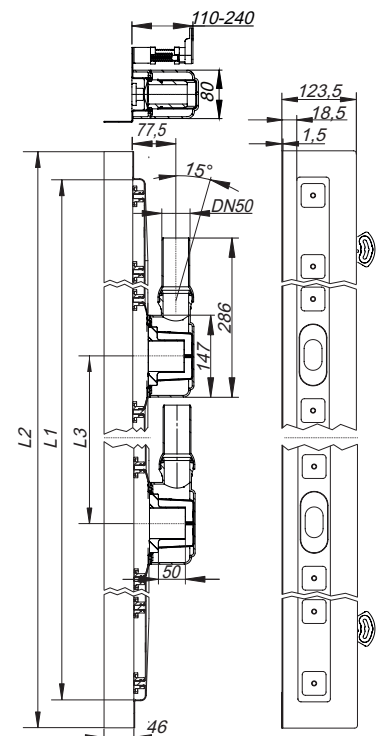
shower channel CeraLine W Duo 1300 – 2000
